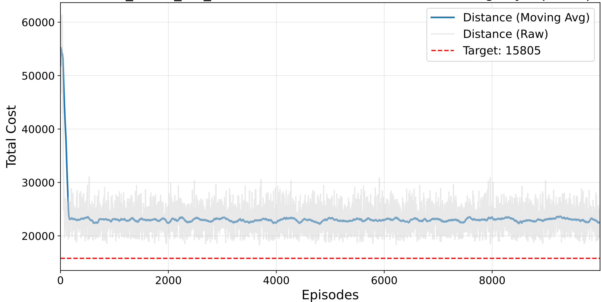
Final NO_MASK_NO_BAYESIAN Masked AutoRL-SOP Training - ry48p.1.sop
